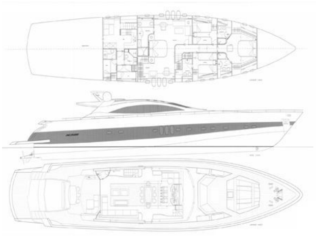
main plan sister ship
