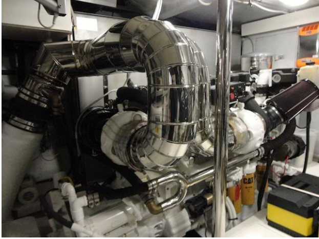
Engines room
