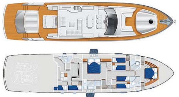
LAYOUT
