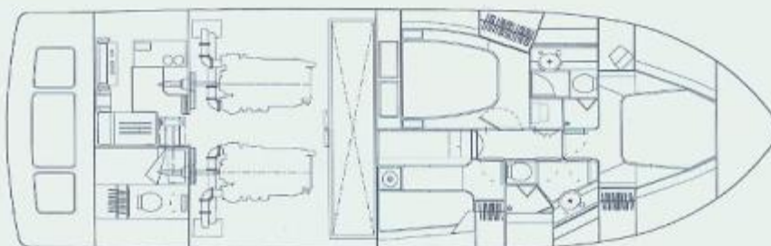
OPTIONAL ARRANGEMENT WITH CREW CABIN AFT
