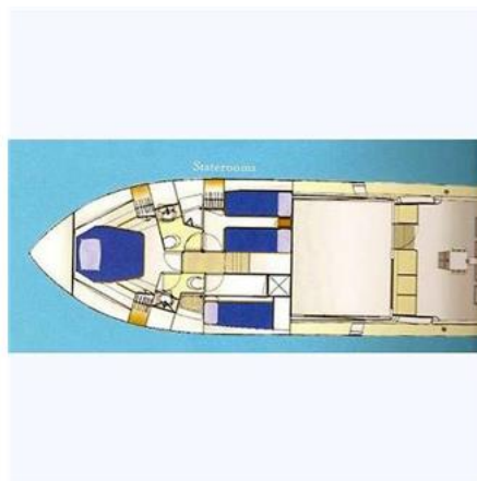
Bertram 450 layout
