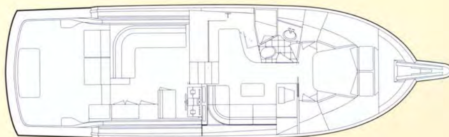
STANDARD ARRANGEMENT*
