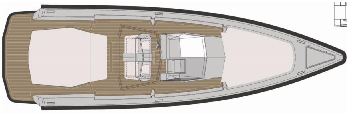
Deck Layout
