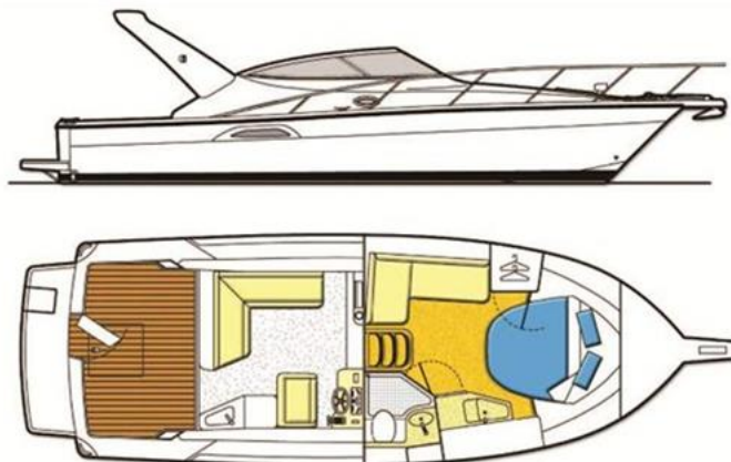
Layout
