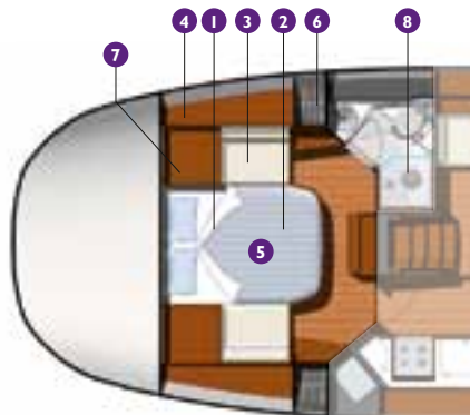
Aft owner's cabin version
