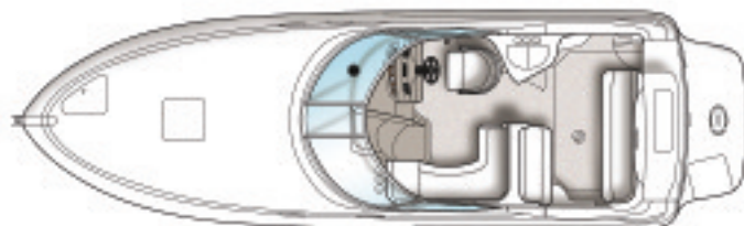
Cockpit Layout
