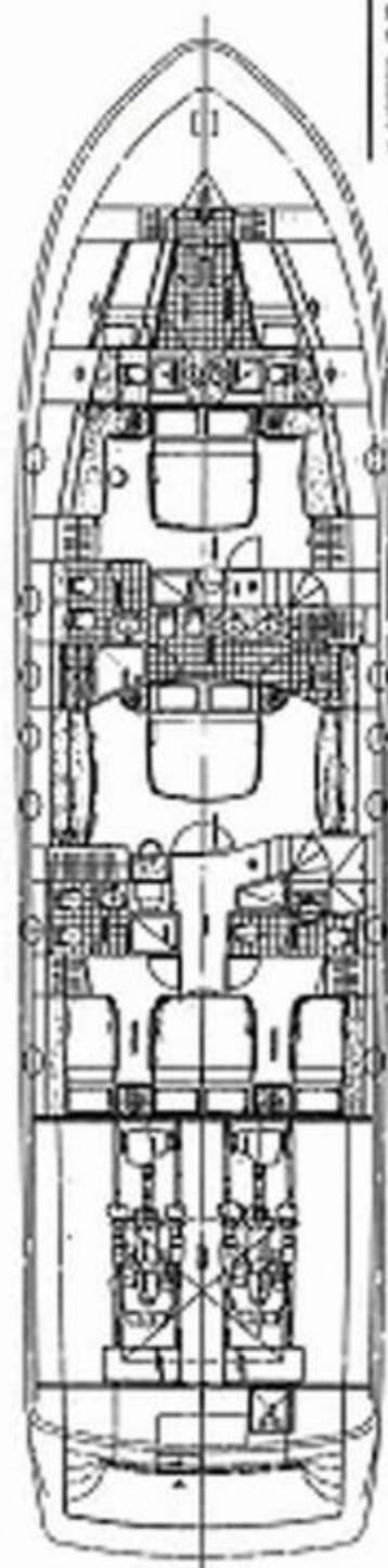
MAIN DECK
