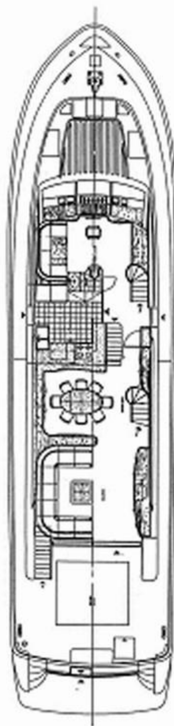
MAIN DECK
