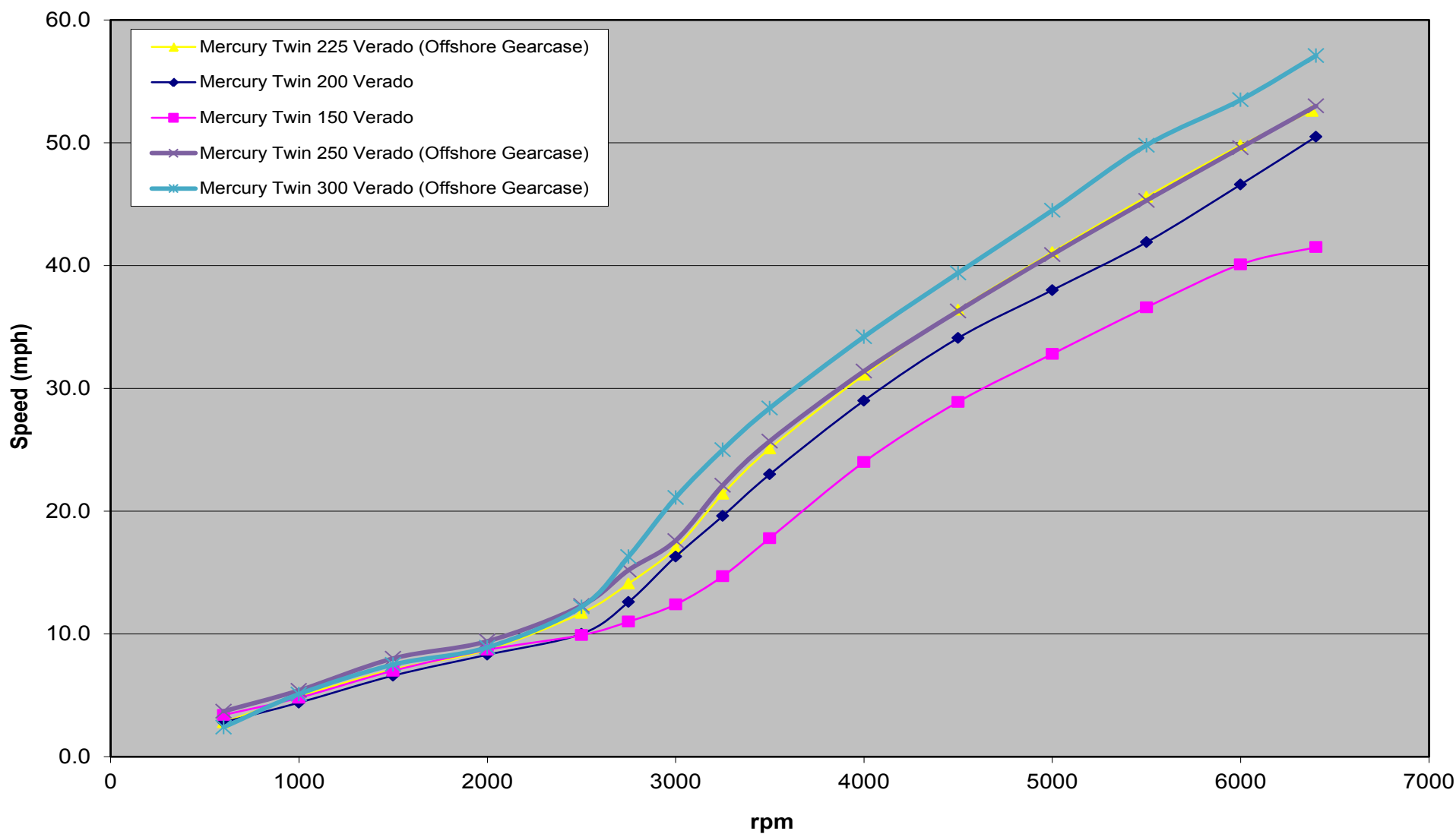
270 Vantage Engine Comparison Graph
