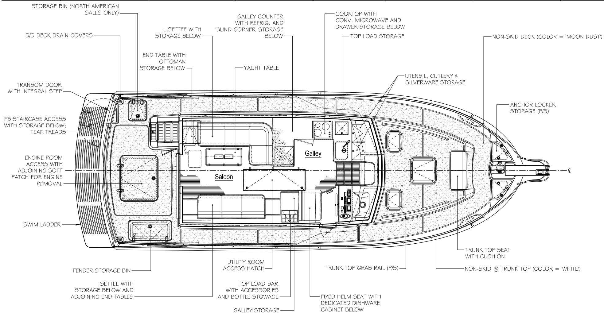
41 Heritage EU \ Standard Main Deck Layout
