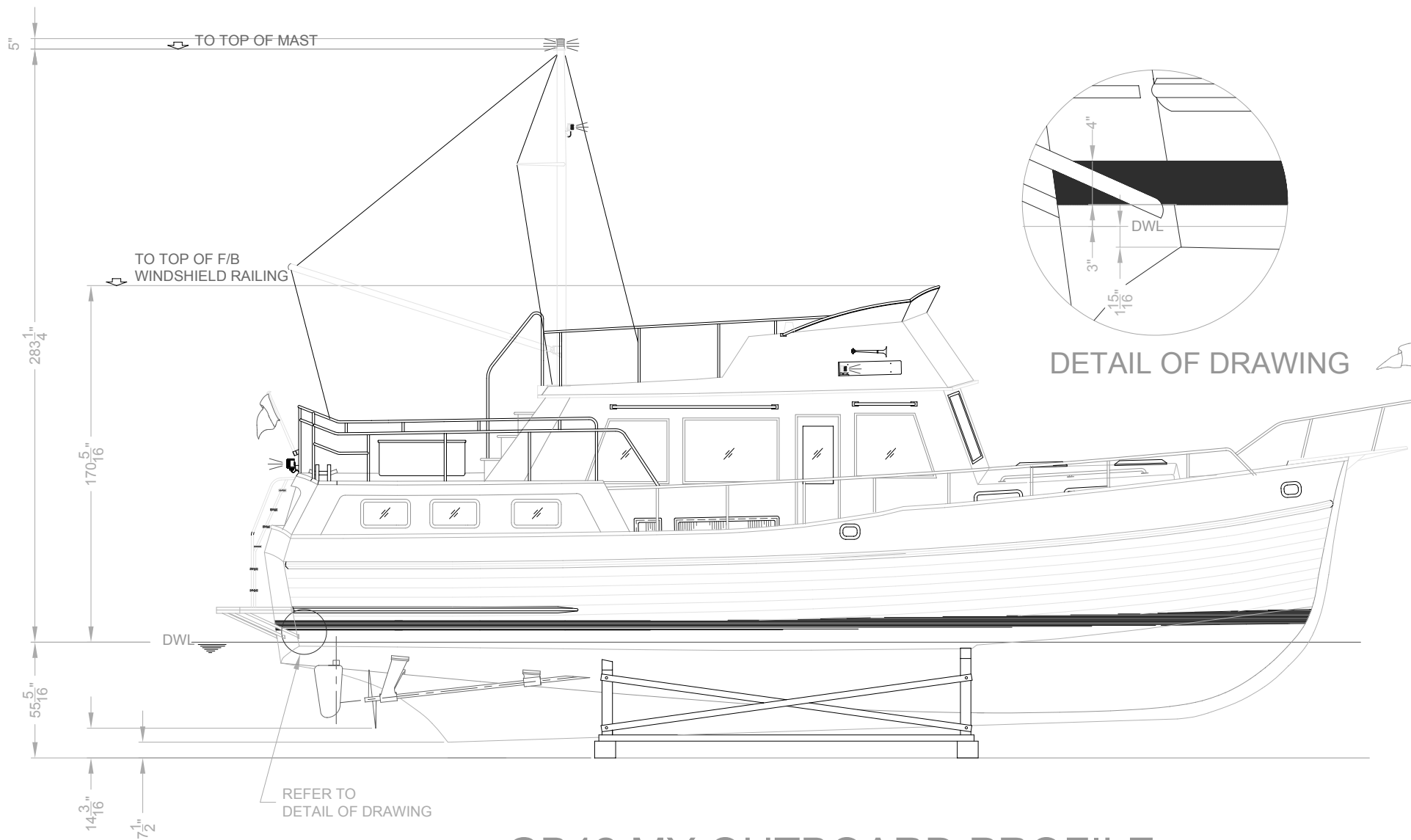
GB42 MY OUTBOARD PROFILE
