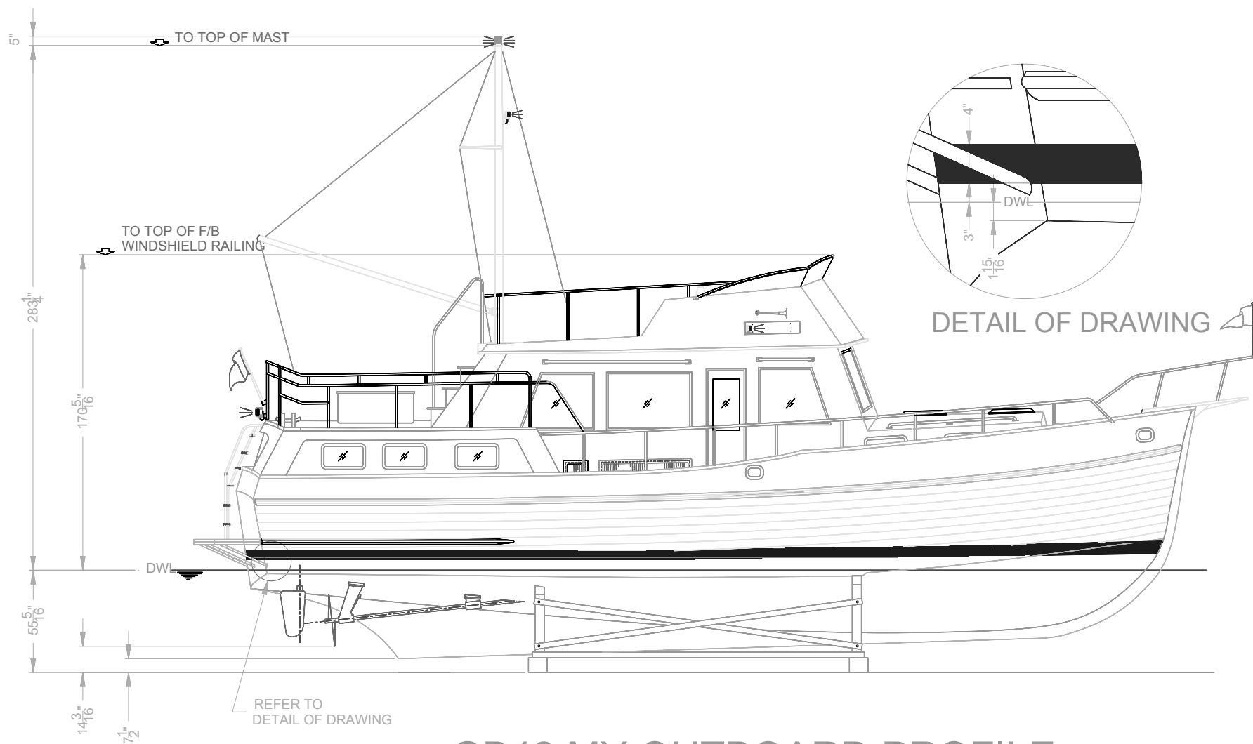
GB42 MY OUTBOARD PROFILE
