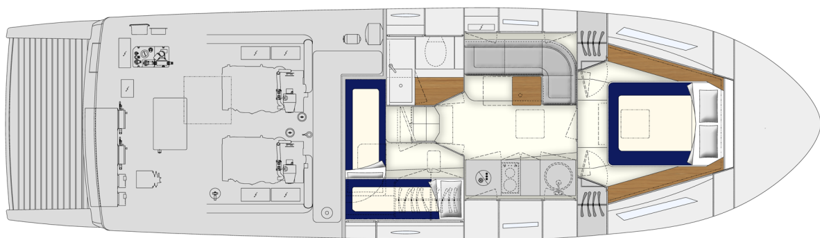
DOUBLE CABIN LAYOUT (STANDARD VERSION)
