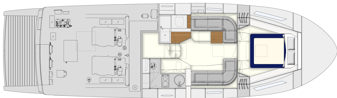
SINGLE CABIN LAYOUT (OPTIONAL VERSION)
