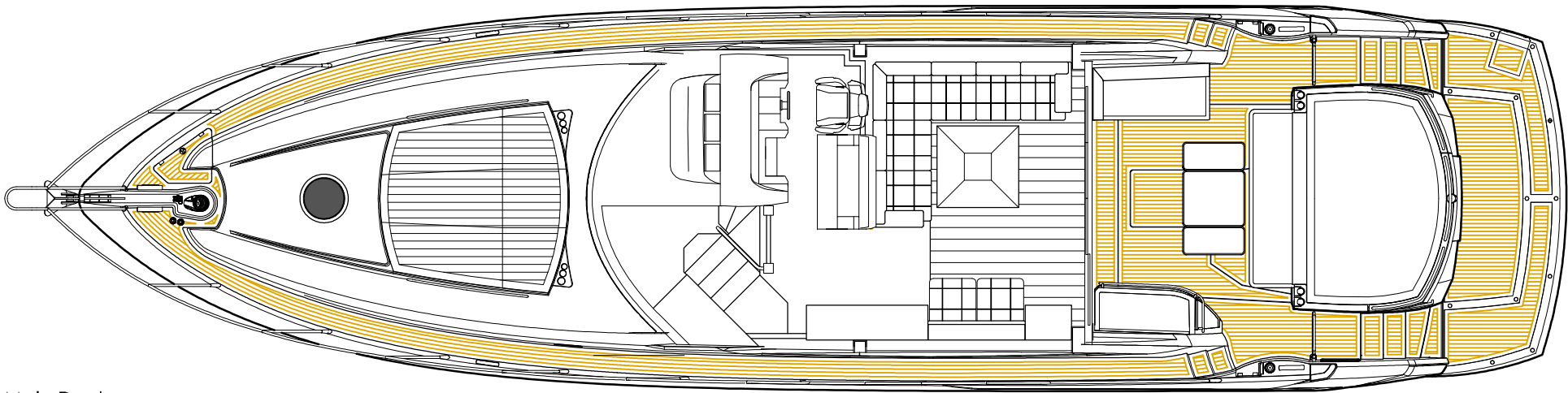
Main Deck
