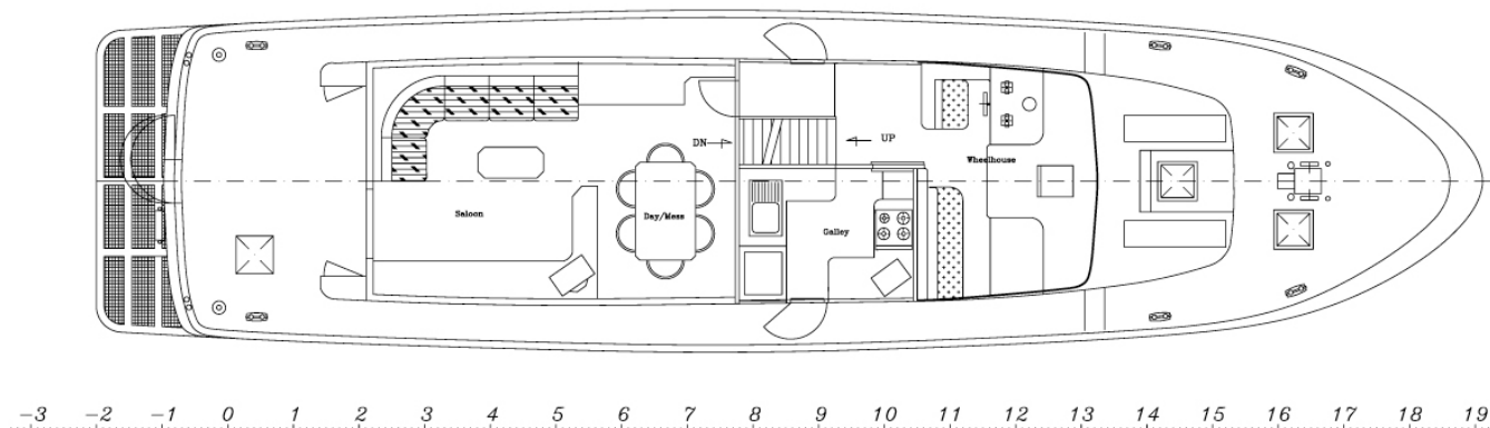
Main Deck
