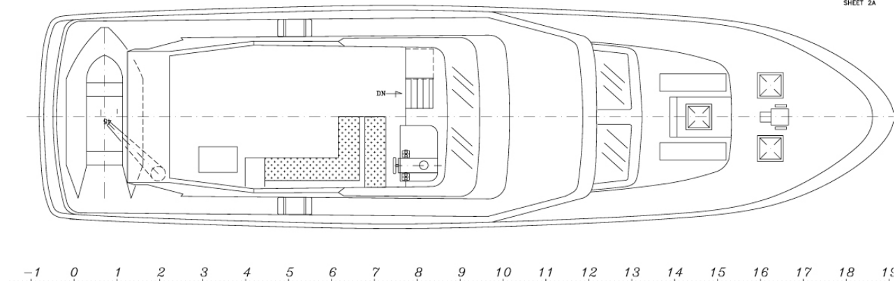
Sun Deck and Fly Bridge
