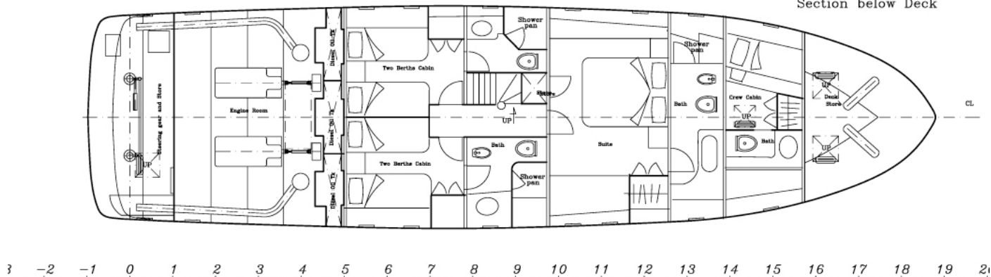
Section below Deck
