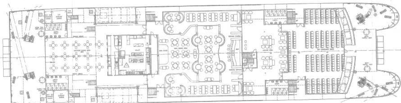
PASSENGER DECK
