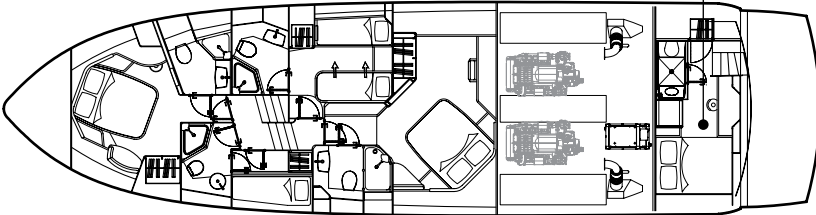
Lower deck
